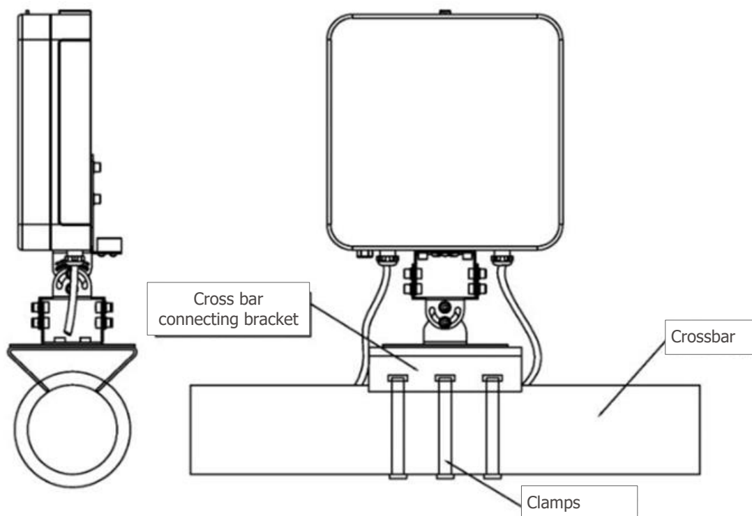
Figure 4 - Radar fixing with clamps
