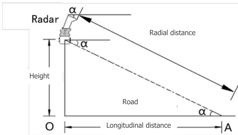
Figure 6 - Schematic diagram of radar adjusting pitch angle
