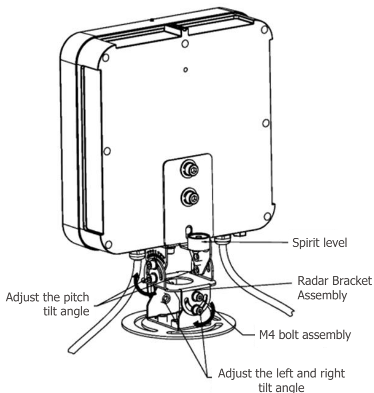
Figure 2 - ITSDETECTOR 24L-3 Radar and Bracket Assembly
