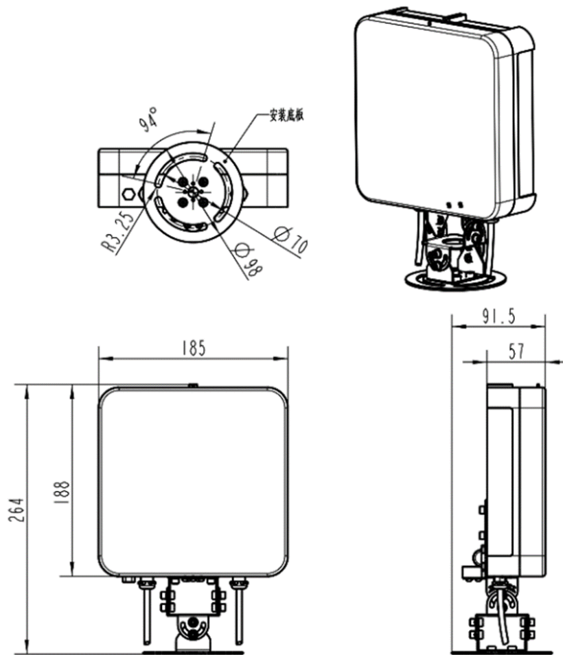
Figure 3 - Radar ITSDETECTOR 24L-3 dimensions
