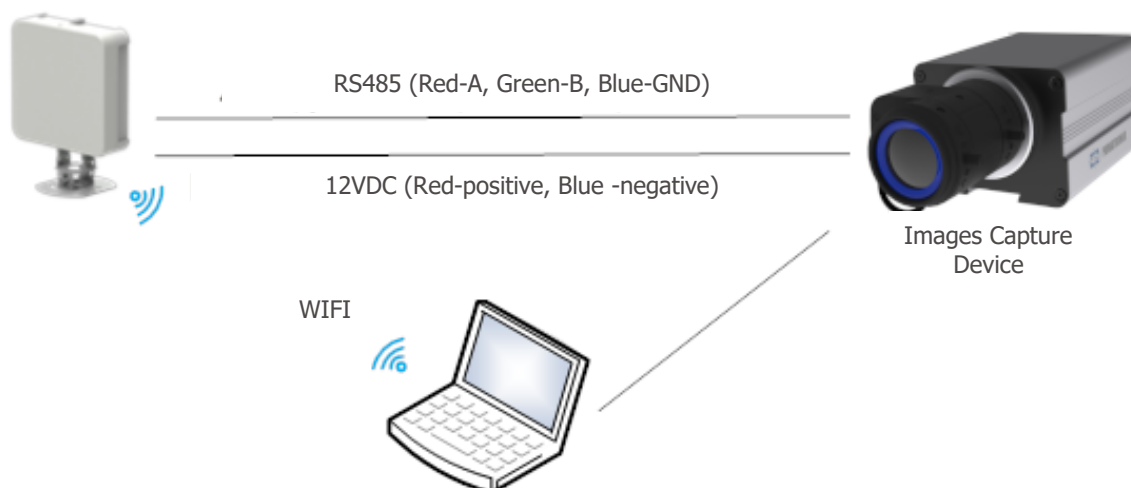
Figure 12 - Diagram of radar connection
