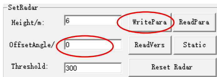
Figure 16 - Installation height and deflection angle settings
