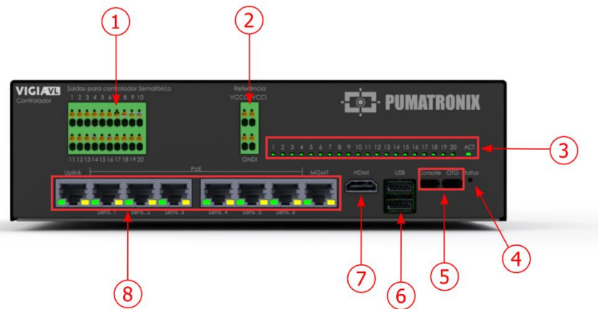
Figure 5 - Interfaces of the New VIGIA-VLIO Controller Module: 1) Outputs for traffic light controller; 2) Connections for powering the IOs; 3) LEDs indicating Output signals; 4) Status LED; 5) microUSB and USB-C inputs; 6) USB input; 7) HDMI input; 8) 6-port PoE Switch
