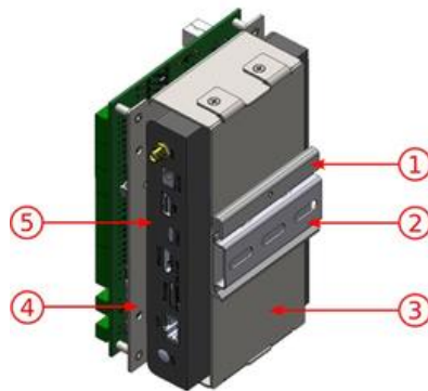
Figure 20– 1) DIN Rail Support; 2) DIN Rail 75mm; 3) Bottom Support; 4) Top Support; 5) ULP
