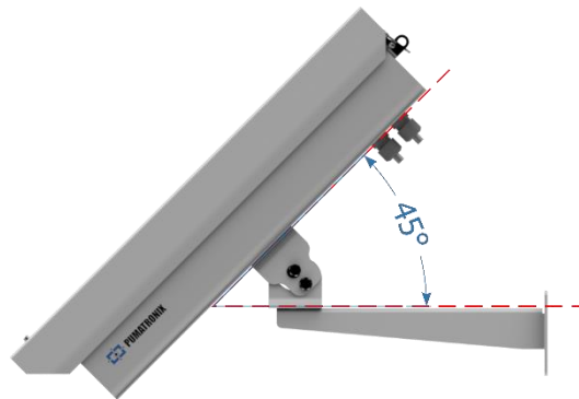
Figure 19 - Maximum angle of inclination of the ITSCAM FF 600 Protection Box
