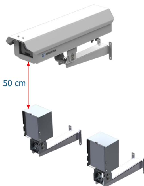
Figure 12 - Example of the installation of 2 illuminators considering the minimum distance from ITSCAM FF 600
