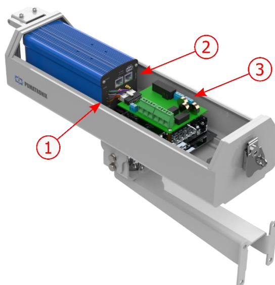
Figure 10 - Connections available on the ITSCAM FF 600* device: 1) Microfit; 2) Ethernet connectors, SMA male for antennas, USB, SD Card and SIM Card; 3) Connectors on the Connection Board
