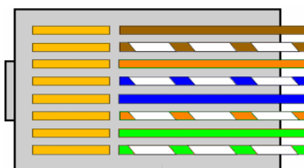
Figure 13 - EIA/TIA-568A standard RJ-45 connector
