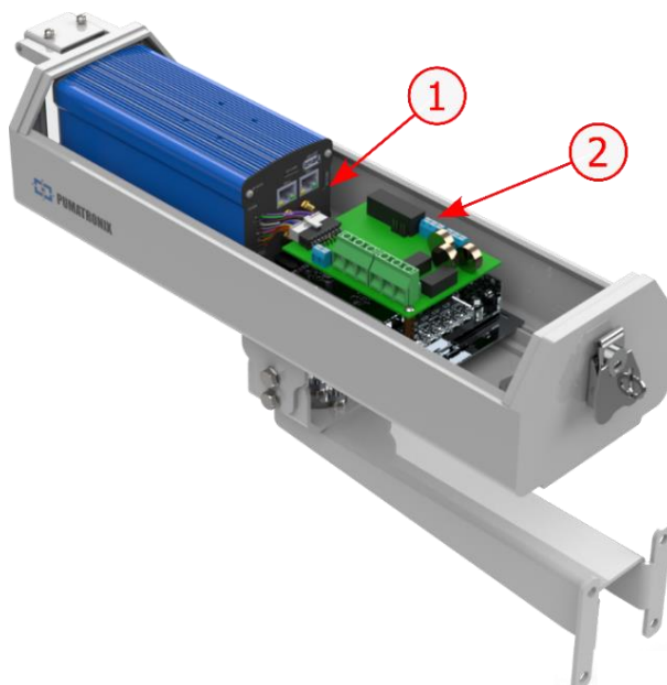
Figure 11 - Available connection interfaces: 1) Connectors on the ITSCAM 600 device; 2) Connectors on the Connection Board
