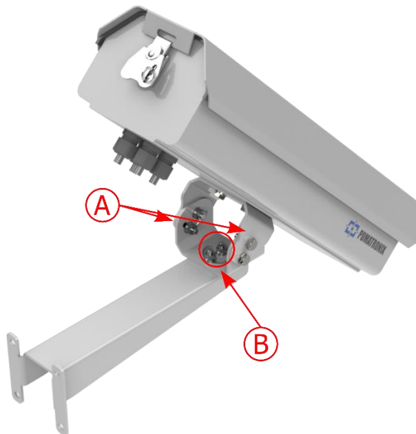
Figure 9 - Possible adjustments to the joint at the base of the equipment: A) Vertical inclination; B) Horizontal rotation
