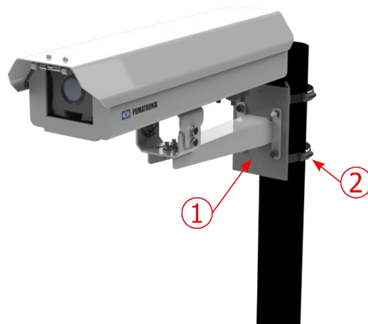
Figure 8 - Poste mounting: 1) Post Bracket; 2) Stainless steel clamp
