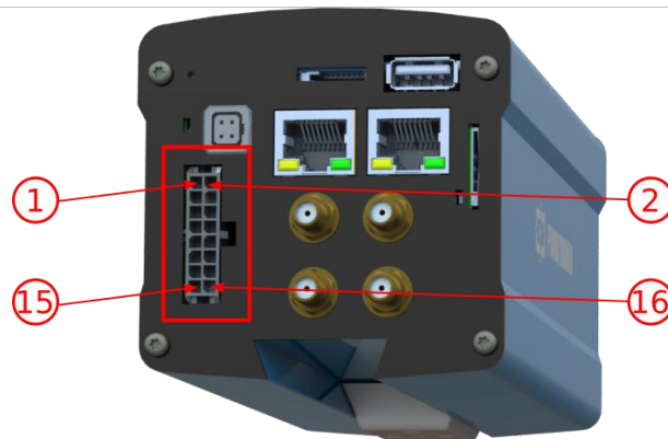
Figure 18 – ITSCAM 600 Power and Signal Connector (Microfit)
