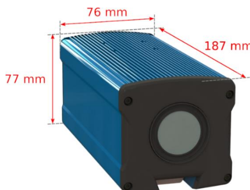
Figura 15 – ITSCAM 600 LM e ITSCAM 600 LM AD IOT
