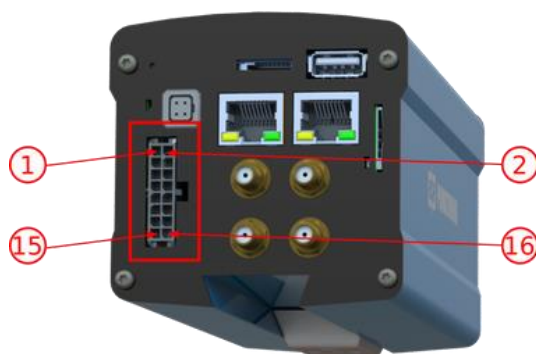
Figure 25 - ITSCAM 600 Power and Signal Connector (Microfit)
