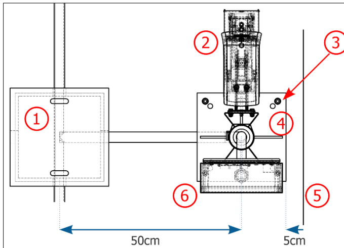
Figure 3 - Panoramic or Rear capture post positioning: 1) Inspection box with cast iron cover, 2) ITSCAM VIGIA+ fixed to the post, 3) Parabolt type anchor bolts, 4) Post base, 5) Existing sidewalk curb, 6) Terminal box fixed to the post
