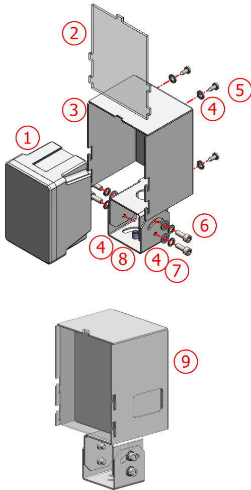
Figure 9 - ITSLUX NEVADA Bracket Parts
