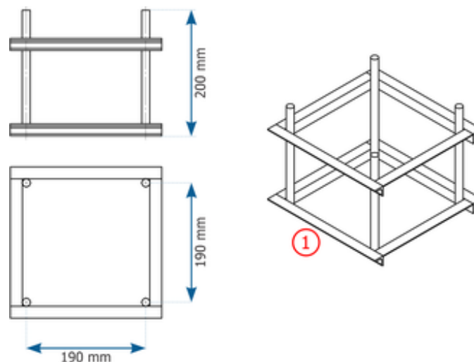
Figure 4 - Anchor Dimensions 190mm (1)
