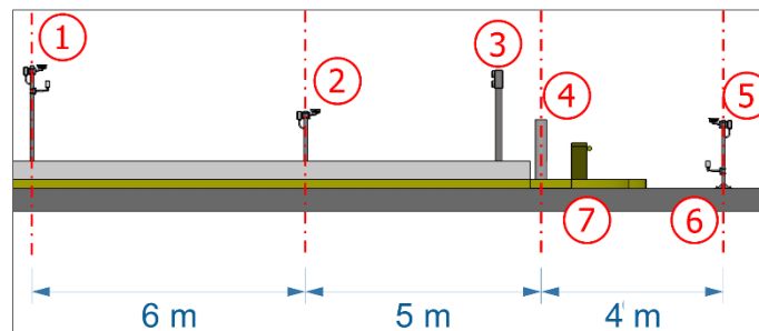
Figure 2 - Side view of the installation in an automatic toll lane (AVI): 1) Panoramic capture post, 2) Rear capture post, 3) Track traffic light, 4) Track optical barrier, 5) Front capture post, 6) Track loop, 7) Track barrier
