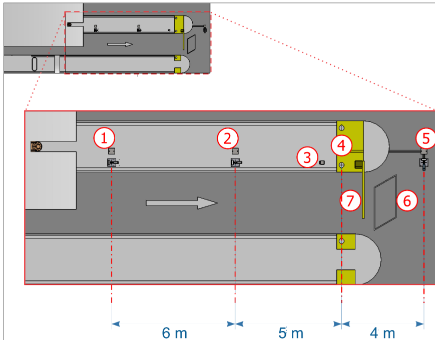
Figure 1 - Top view of the installation in an automatic collection lane (AVI): 1) Panoramic capture post, 2) Rear capture post, 3) Track traffic light, 4) Track optical barrier, 5) Front capture post, 6) Runway loop, 7) Track barrier
