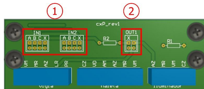
Figure 20 - Connections available on the Terminal Box plate: 1) Input Signals, 2) Output Signal
