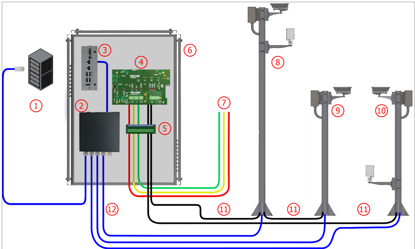
Figure 14 - NEVADA Installation Diagram on a Track: 1) Utility network, 2) Switch, 3) ULP - Local Processing Unit, 4) Supervisory Board, 5) General Connector, 6) NEVADA Frame or NEVADA Compact Frame, 7) Signals from Track, 8) Panoramic Image Post, 9) Rear Image Post, 10) Front Image Post, 11) 8x22AWG shielded sleeve cable, 12) Furukawa External CAT-5E Cable
