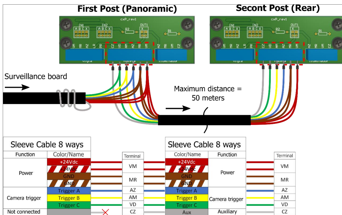
Figure 18 - Wiring Diagram for the 8-way sleeve cable in each Junction Box of the Panoramic and Rear Capture Posts
