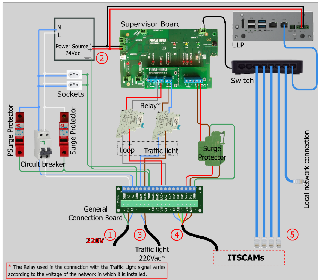
Figure 26 - NEVADA Compact Frame Wiring Diagram
