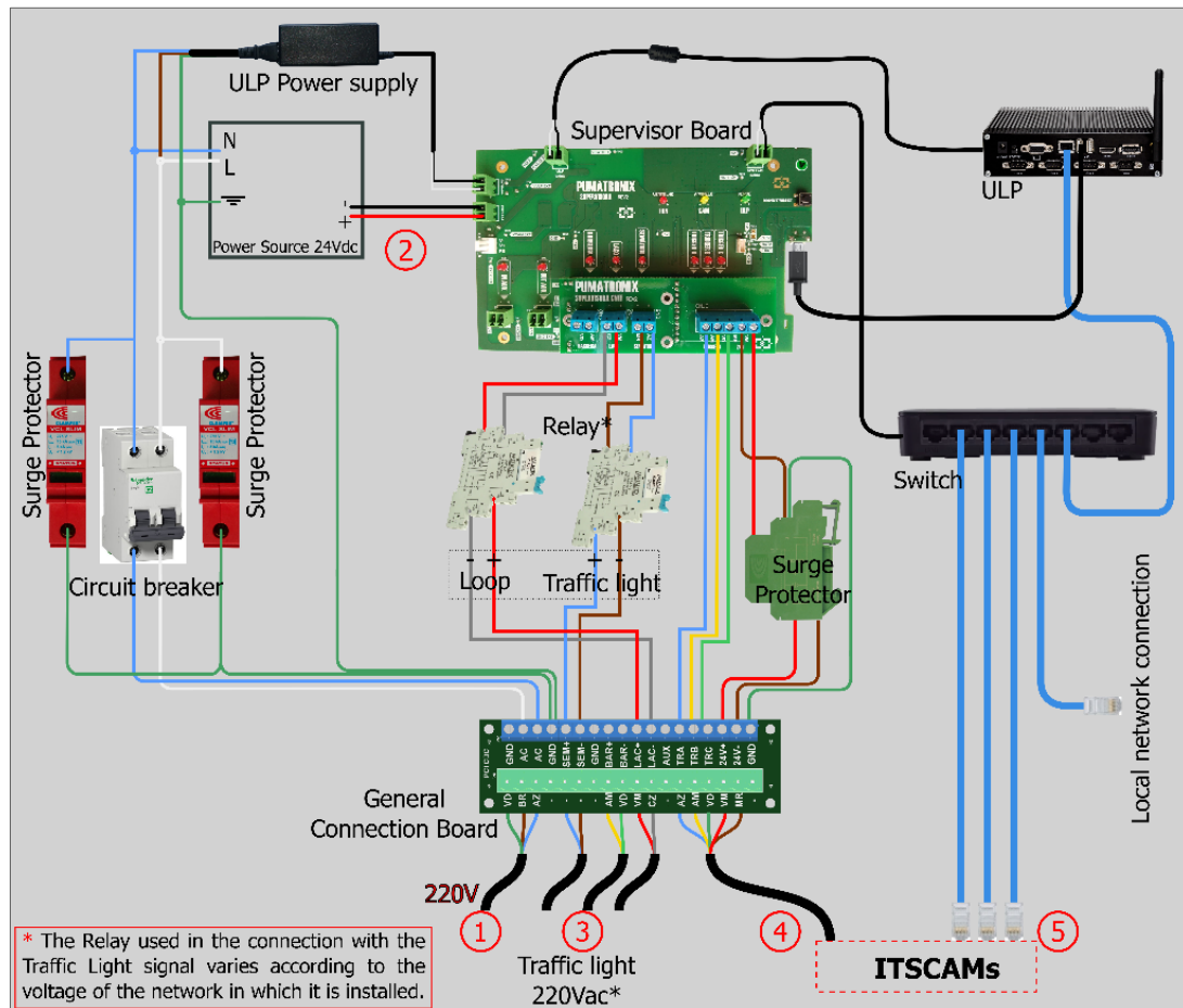
Figure 25 - NEVADA Panel Connection Diagram
