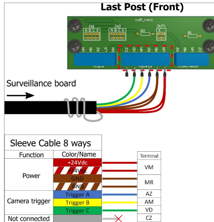
Figure 19 - Wiring Diagram for the 8-Core Sleeve Cable in the Front Catchment Post Junction Box
