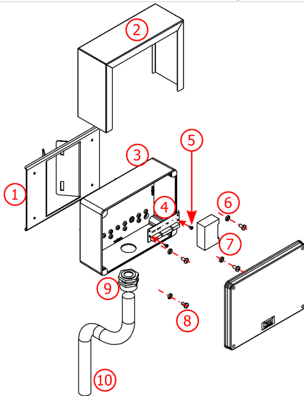
Figure 6 - Terminal box components
