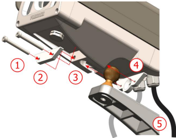
Figure 7 - VIGIA+ Bracket Parts
