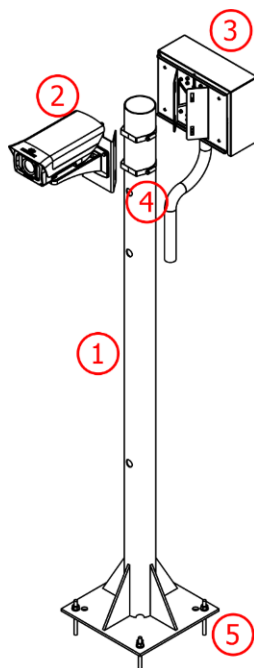
Figure 12 - Rear Image Capture Post
