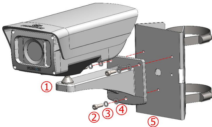
Figure 8 - VIGIA Post Bracket Parts
