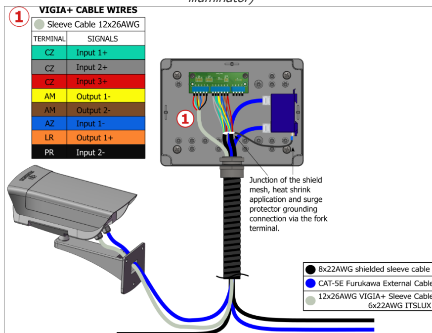
Figure 16 - Connection Diagram for ITSCAM VIGIA+ device on Rear or Panoramic Post (without illuminator)
