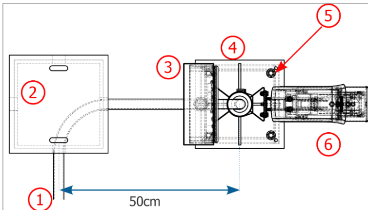
Figure 5 - Positioning of Frontal capture post on asphalt: 1) Cable protection piping, 2) Inspection box with cast iron cover, 3) Terminal box fixed to the post, 4) Post base, 5) Fastening point to the 190mm anchor bolt, 6) ITSCAM VIGIA+ fixed to the post
