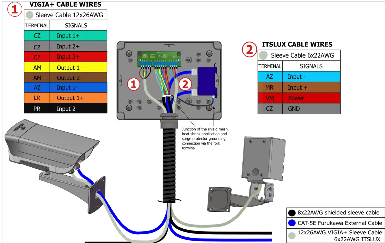
Figure 15 - Connection diagram of the ITSCAM VIGIA+ and ITSLUX devices in the Panoramic Post (with illuminator)
