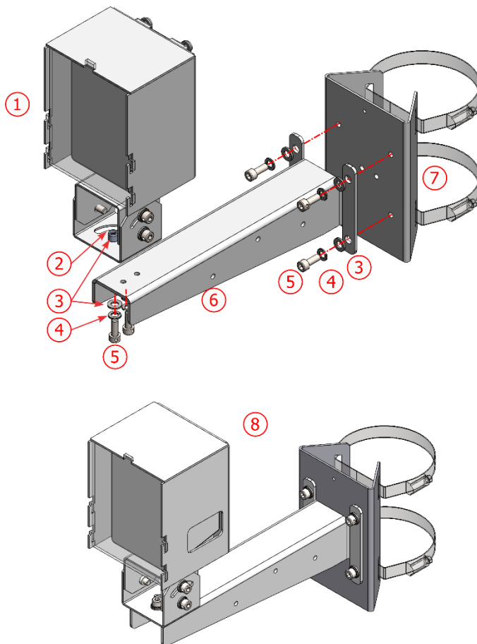
Figure 10 - Parts for fastening the ITSLUX NEVADA Bracket to the Post Bracket
