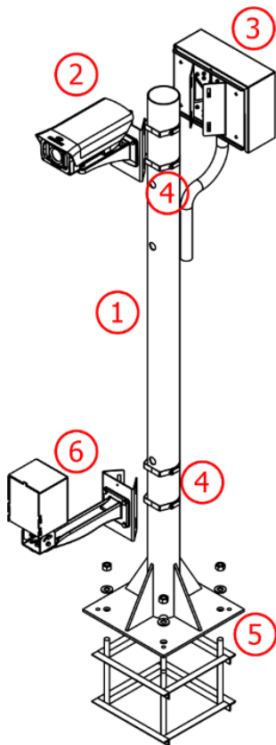
Figure 13 - Front Image Capture Post
