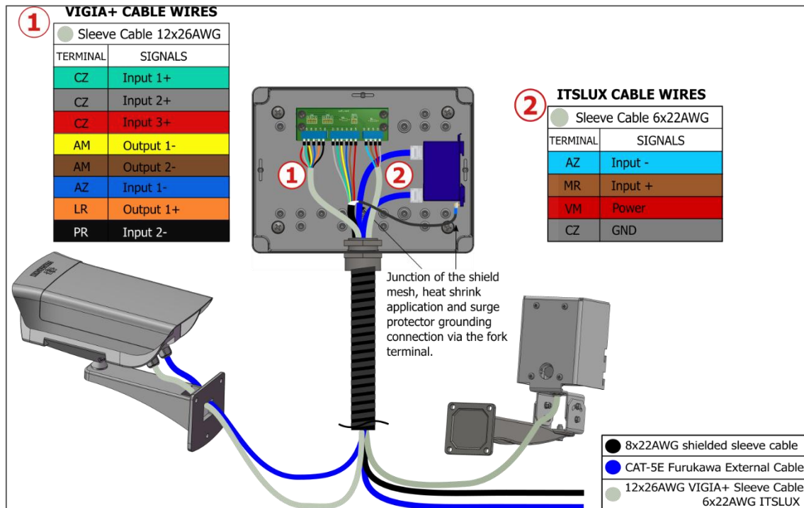
Figure 17 - Connection Diagram for ITSCAM VIGIA+ and ITSLUX devices on the Front Post
