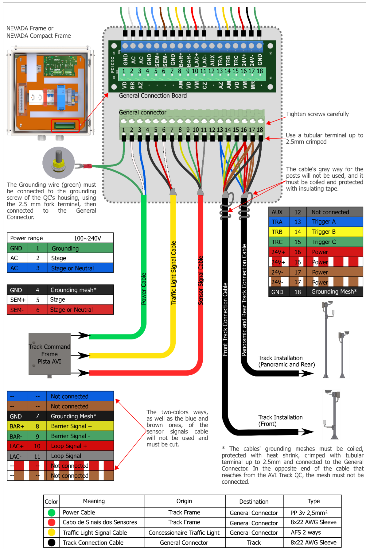
Figure 24 - Connection Diagram with the General Connection Board
