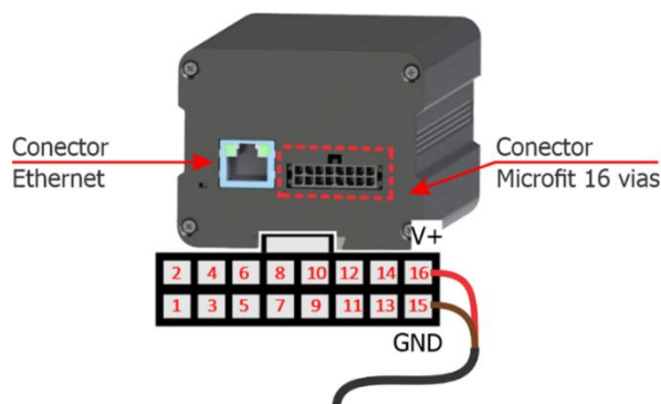
Figure 18- Connections to the Secondary Module Device: 1) Ethernet cable; 2) 8-way sleeve cable
