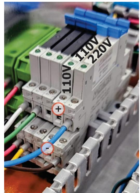
Figure 14 – 110V relay connections to the General Connection Board
