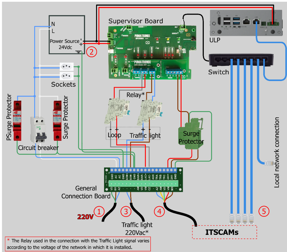
Figure 12 - Connection diagram with the Surveillance Board on the Compact NM1 Switchboard (when 220 Vac Traffic Light)
