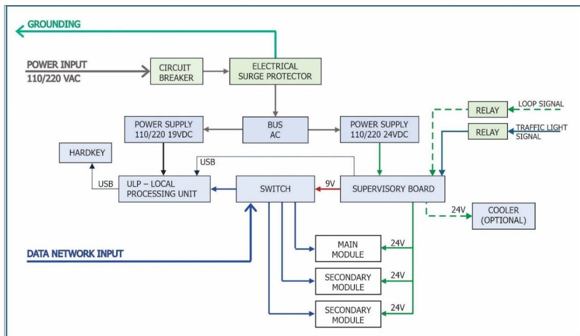
Figure 8 - NM1 Switchboard Installation Diagram
