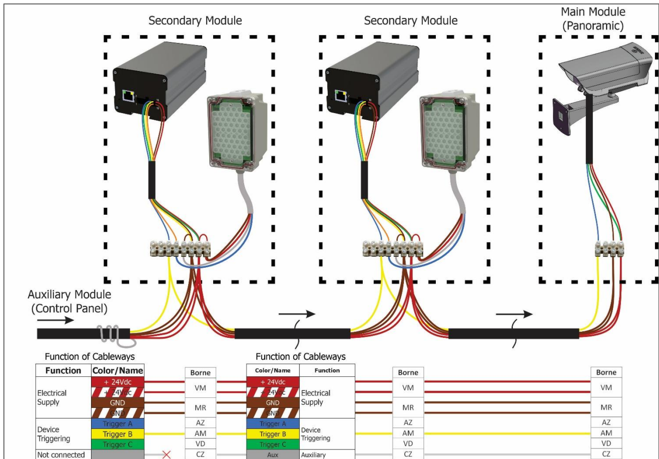
Figure 16 – Module Connections Diagram
