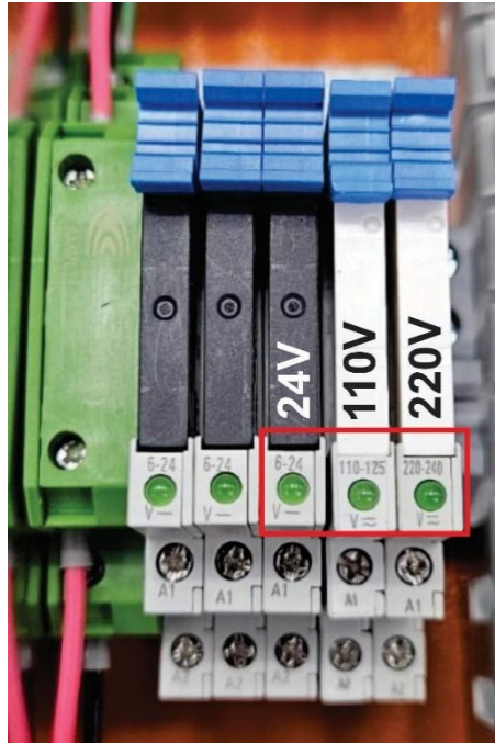
Figure 13 – Voltage of the relays available for connecting the traffic light signal
