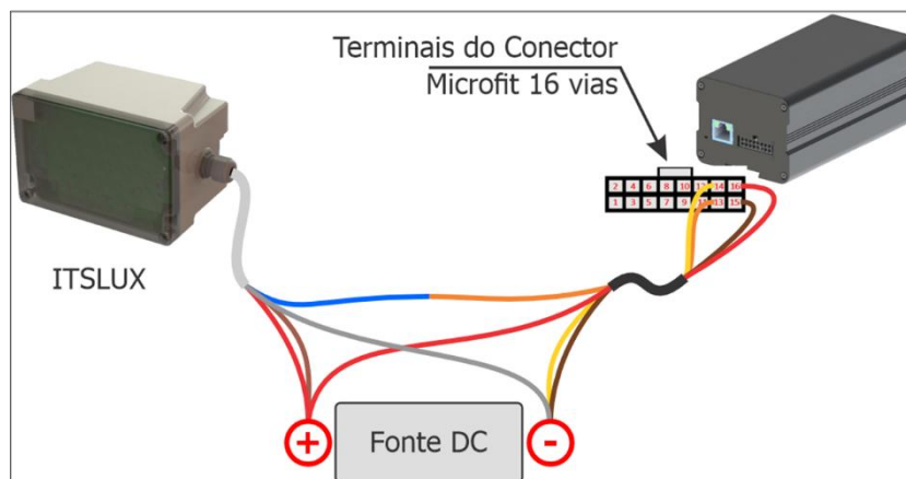
Figure 19 - Diagram illustrating the connections between the ITSCAM device and the ITSLUX Illuminator
