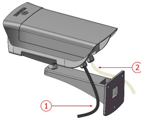
Figure 17- Connections to the Main Module Device: 1) Ethernet cable; 2) 8-way sleeve cable
