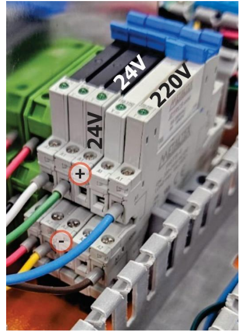
Figure 15 - 24V relay connections to the General Connection Board
