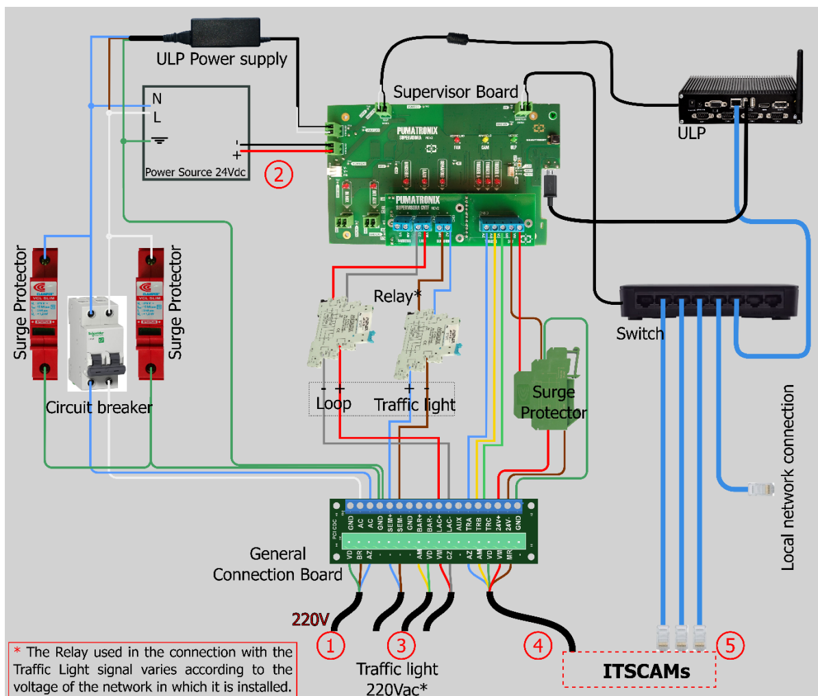
Figure 11 - Connection diagram with the Surveillance Board from NM1 Switchboard (when 220 Vac Traffic Light)
