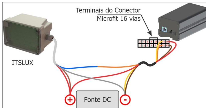
Figure 16 - Diagram illustrating the connections between the ITSCAM device and the ITSLUX Illuminator
