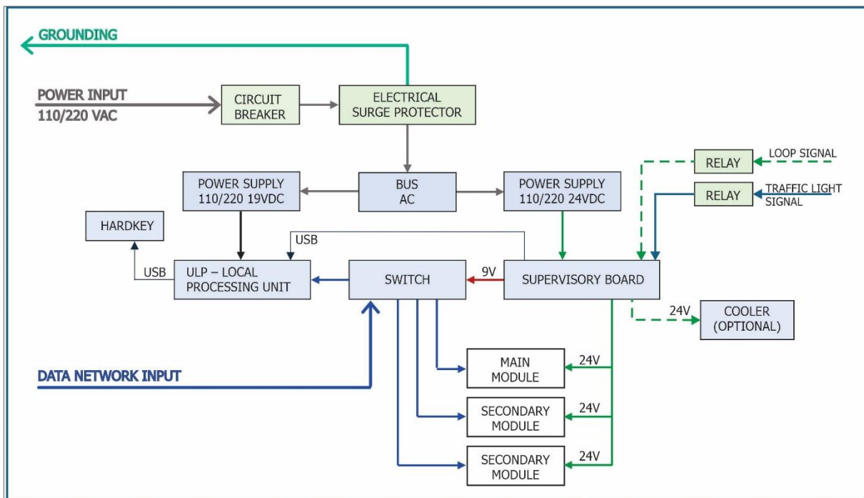
Figure 8 - NM1 Switchboard Installation Diagram
