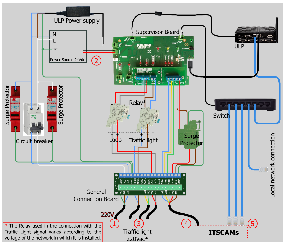
Figure 11 - Connection diagram with the Surveillance Board (when 220 Vac Traffic Light)
