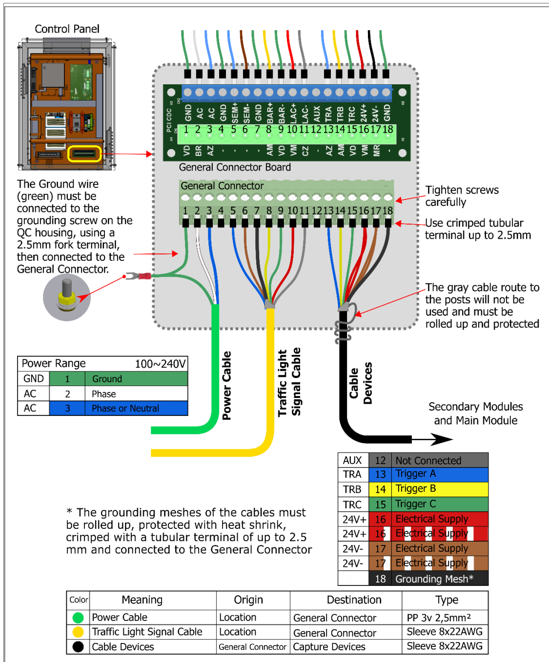
Figure 10 – Tertiary Module General Connector Diagram
