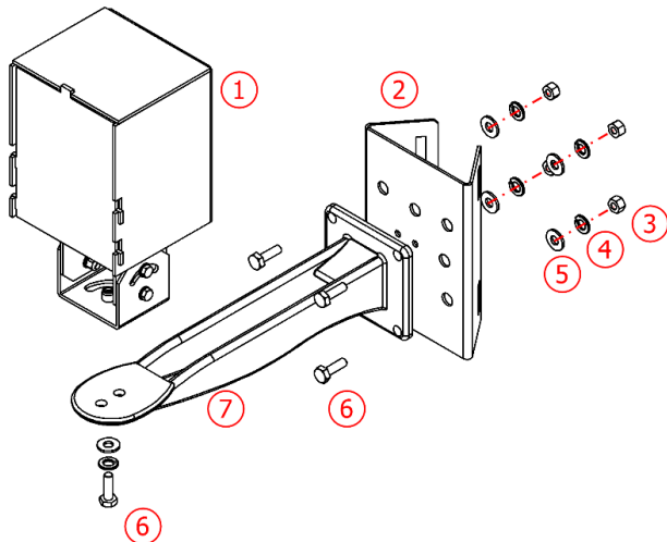
Figure 6 - ITSLUX Illuminator Cage Bracket Parts
