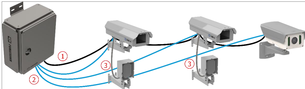
Figure 3 – General wiring diagram for cables and devices: 1) 8-way sleeve cable; 2) Ethernet cables; 3) ITSLUX cable
