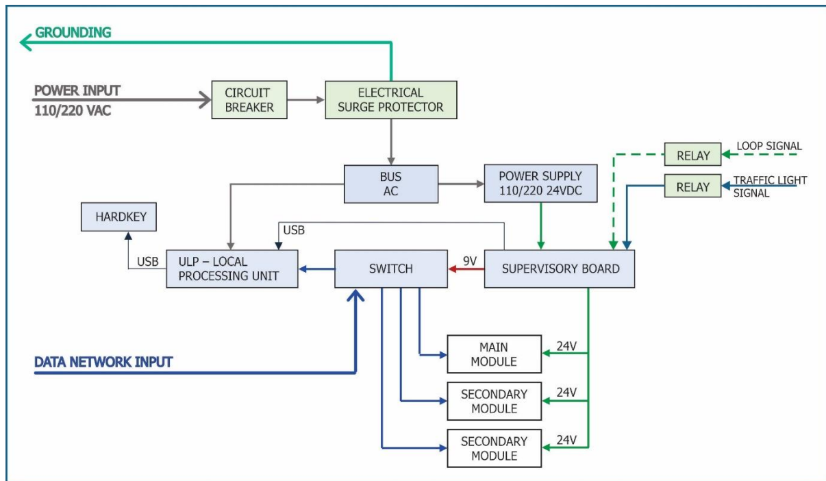
Figure 9 - Compact NM1 Switchboard Installation Diagram
