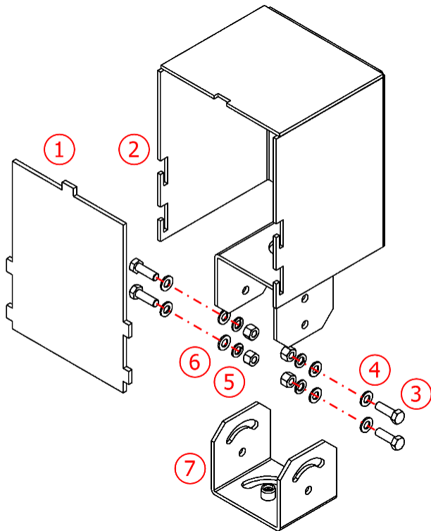
Figure 5 - ITSLUX Bracket Parts
