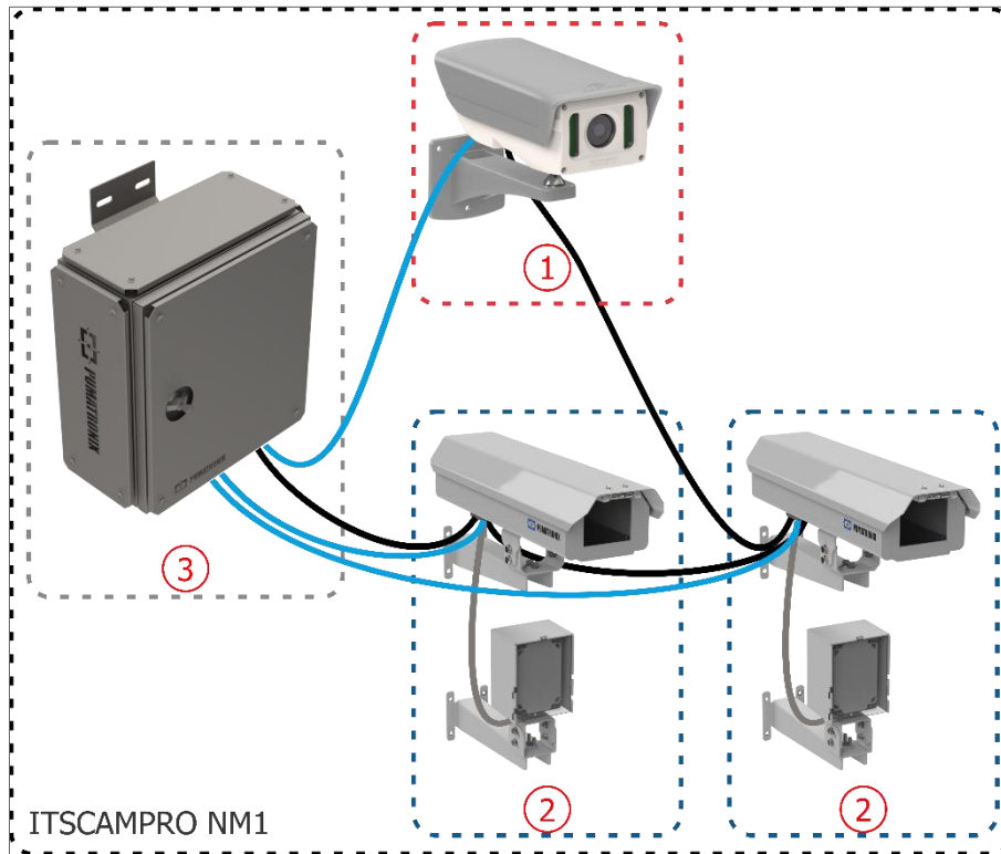
Figure 7 - ITSCAMPRO NM1 General Connection Diagram: 1) Main Module; 2) Secondary Module; 3) Tertiary Module Control Switchboard
