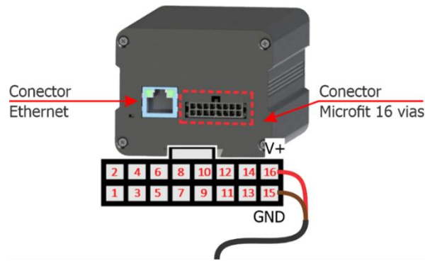
Figure 15- Connections to the Secondary Module Device: 1) Ethernet cable; 2) 8-way sleeve cable
