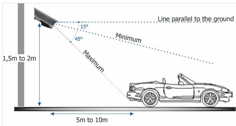
Figure 19 - Side View of the Installation Rear Positioning
