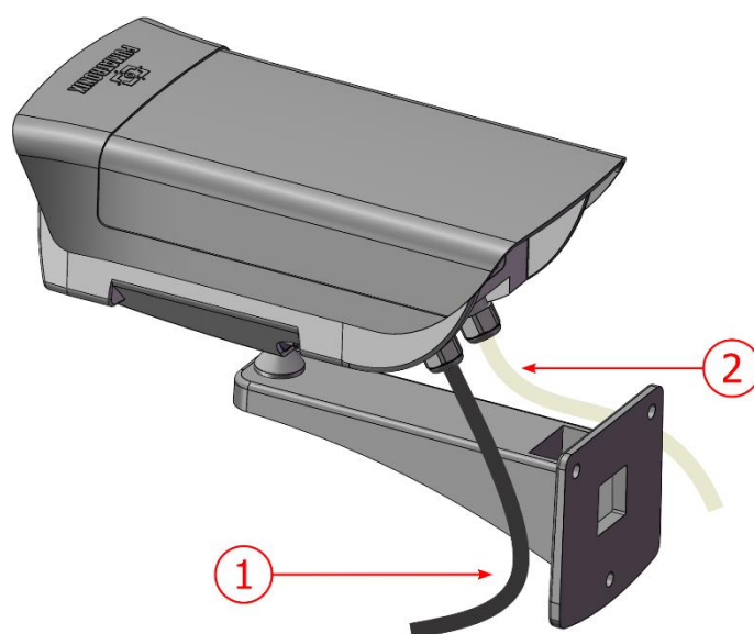
Figure 10 - Cables of the ITSCAM VIGIA+ device housing: 1) Ethernet cable; 2) Multi-way cable
